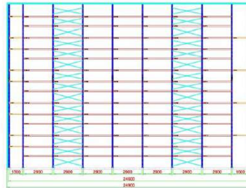
D-D View
