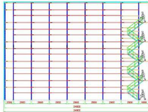
B-B View
