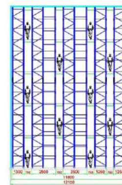
F-F View
