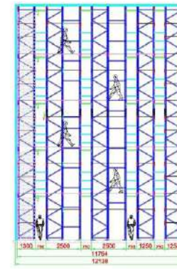
G-G View
